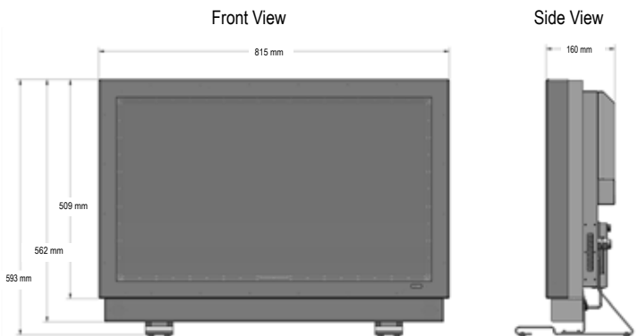
SunBriteTV Model SB3220HD (All dimensions are in millimeters)
